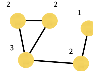
Node degrees
